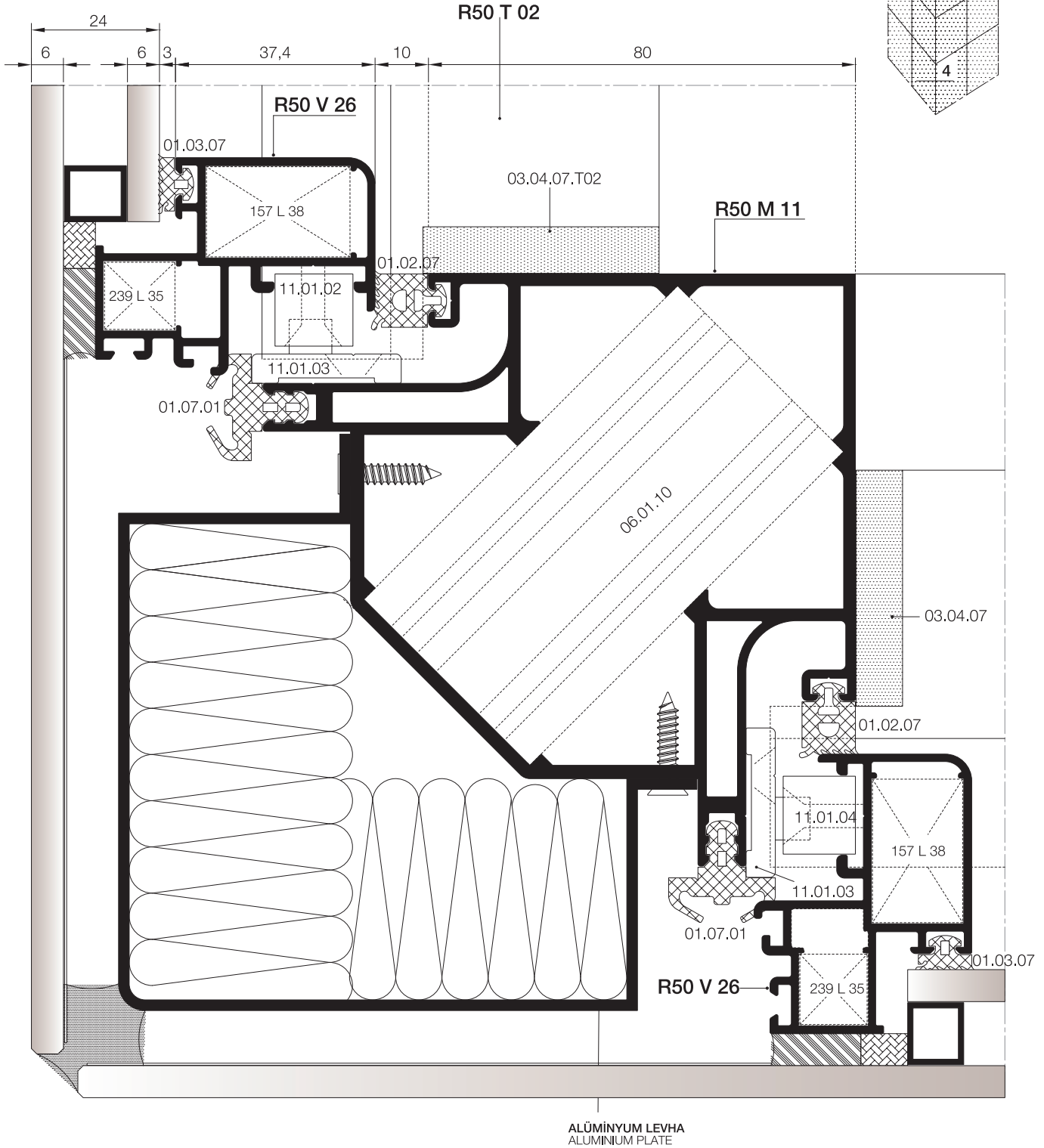
SİLİKON CEPHE KÖŞE DÖNÜŞ DETAYI STRUCTURAL GLAZING CORNER DETAIL
