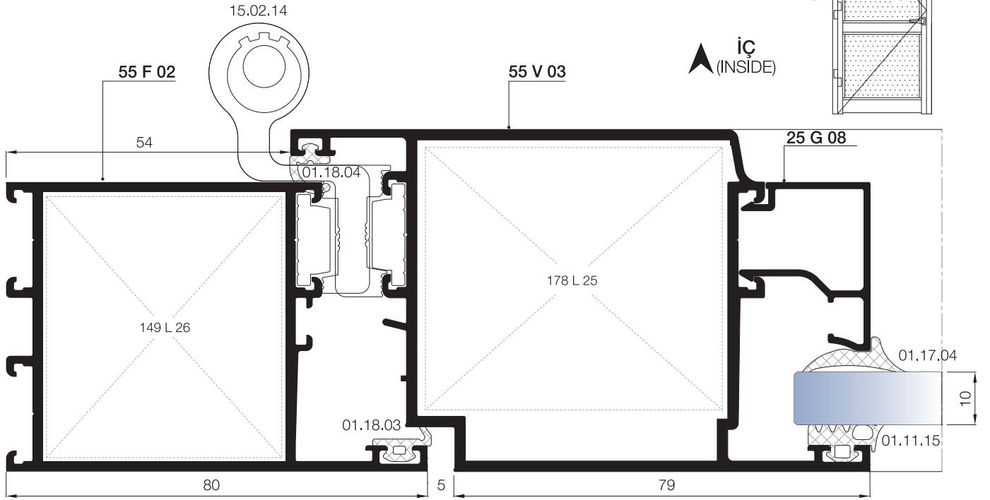
19 DETAYI DETAIL
