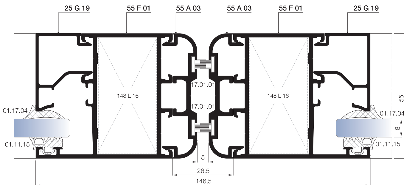
15 DETAYI DETAIL
