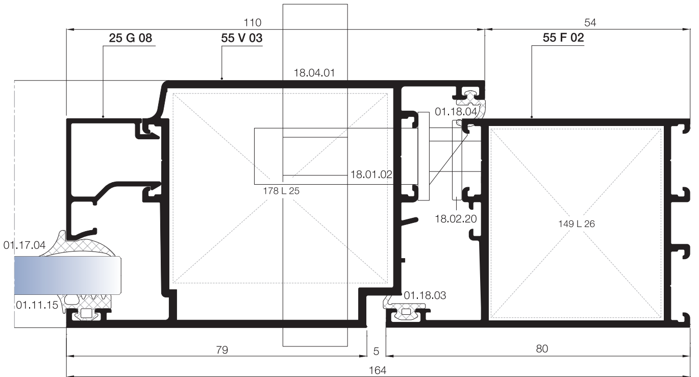
20 DETAYI DETAIL
