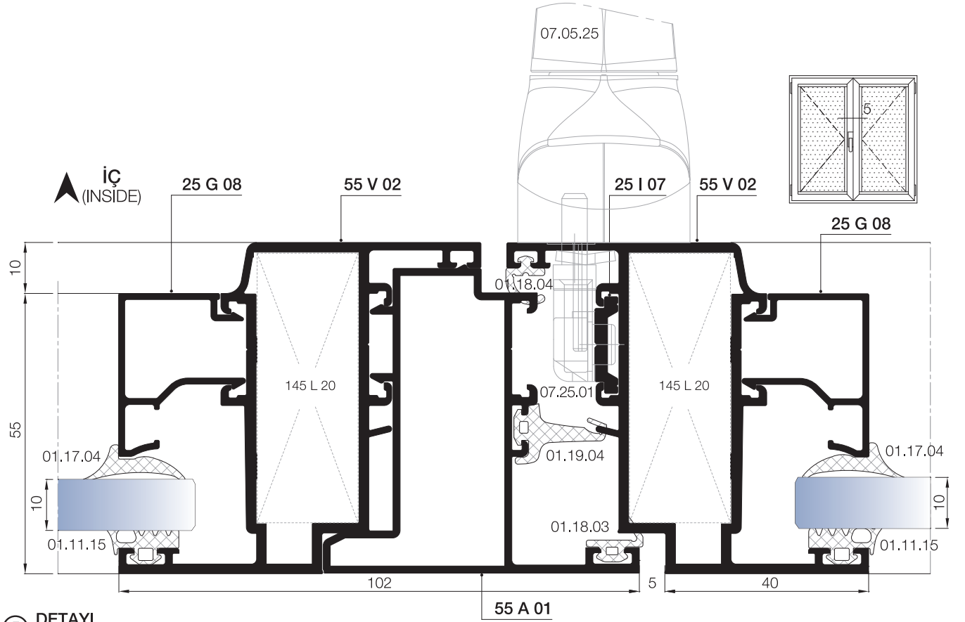
5 DETAYI DETAIL
