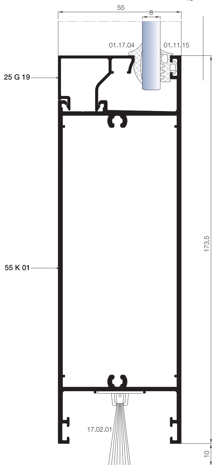
18 DETAYI DETAIL
