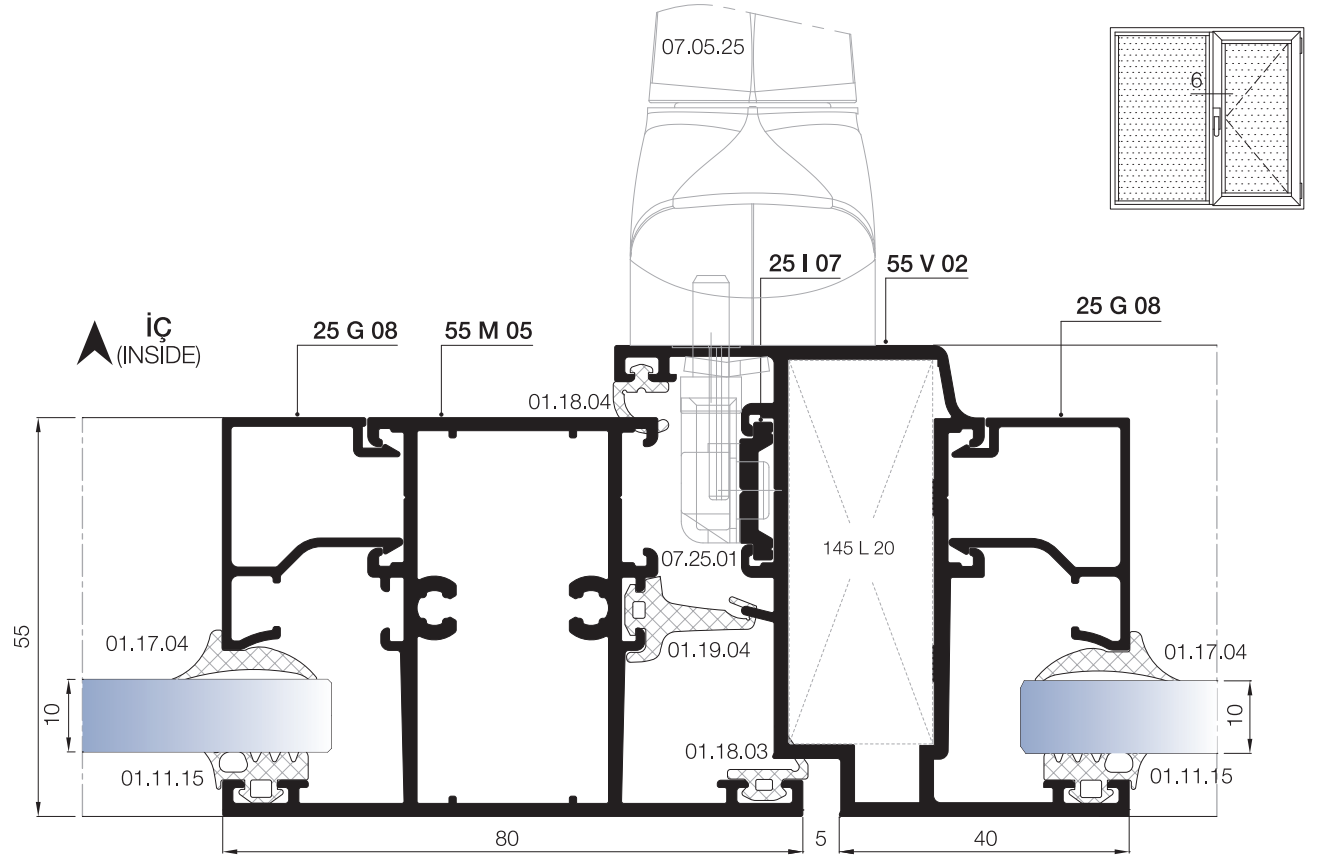
6 DETAYI DETAIL
